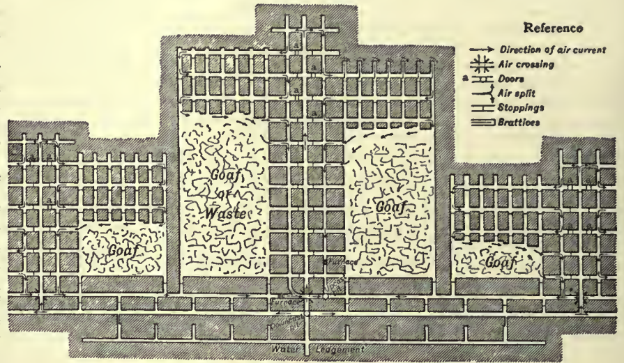
FIG. 5.—Pillar Working.
